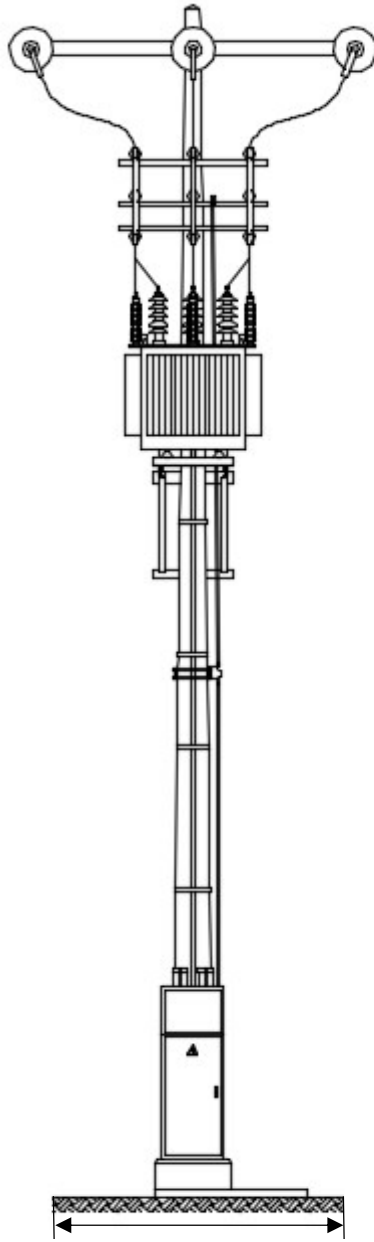
VISTA FRONTAL
